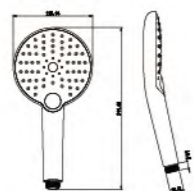
YS31418 ABS handshower Size: \phi 120mm
